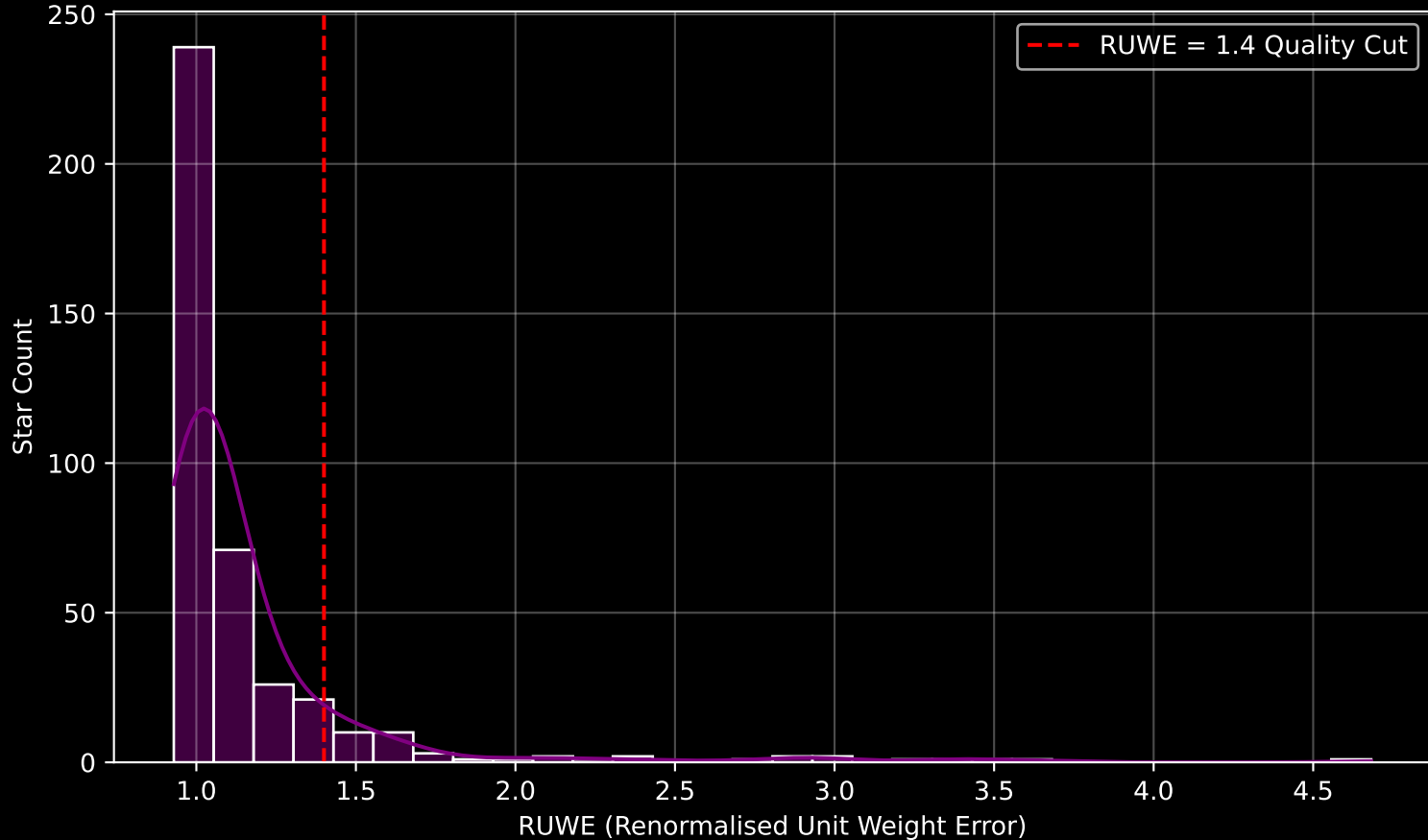
GAPOGEE DR17 Field [150+30] RUWE Distribution (n= 397)
