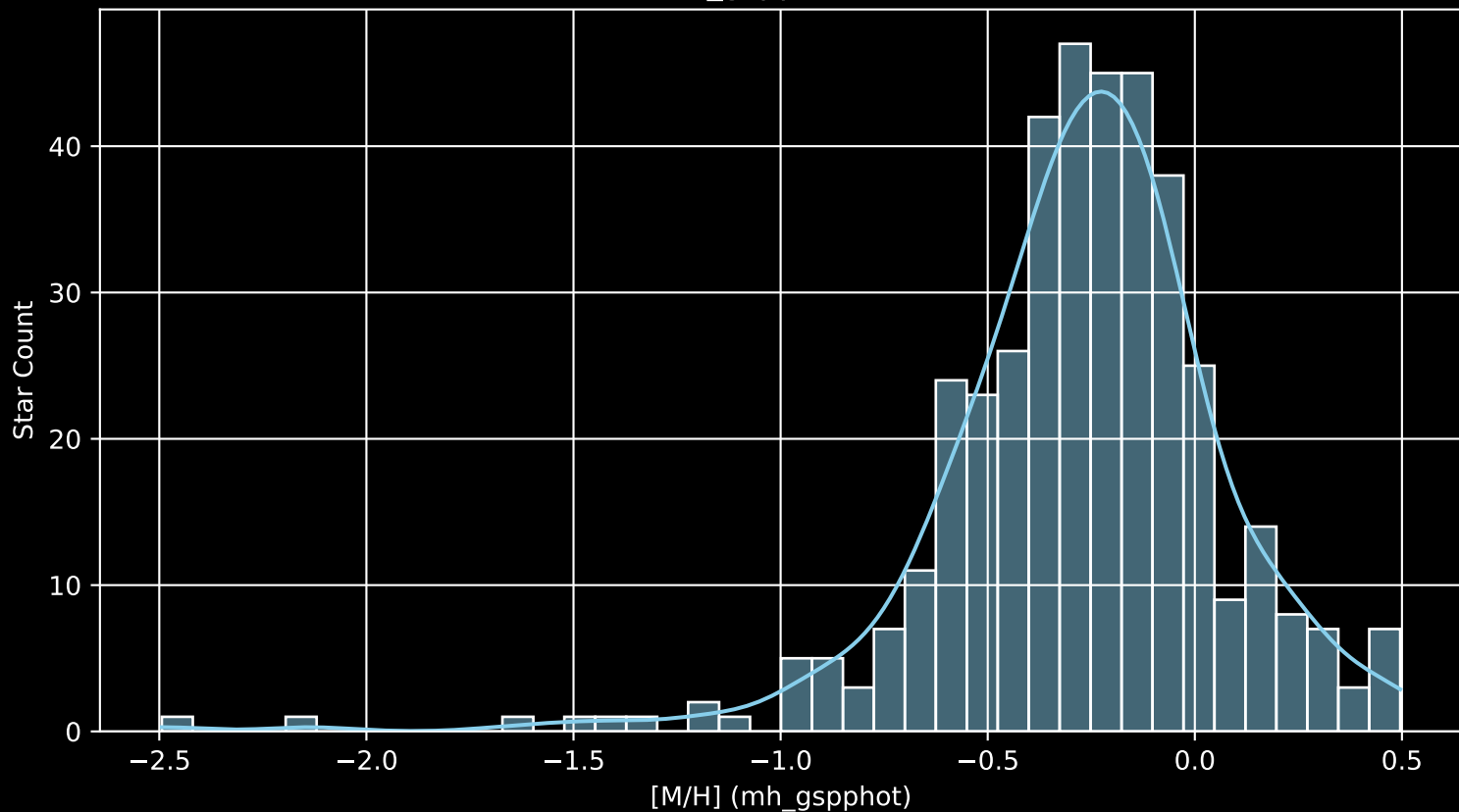
APOGEE DR17 Field: [150+30 [M/H] (mh_gspphot) (n= 403)
