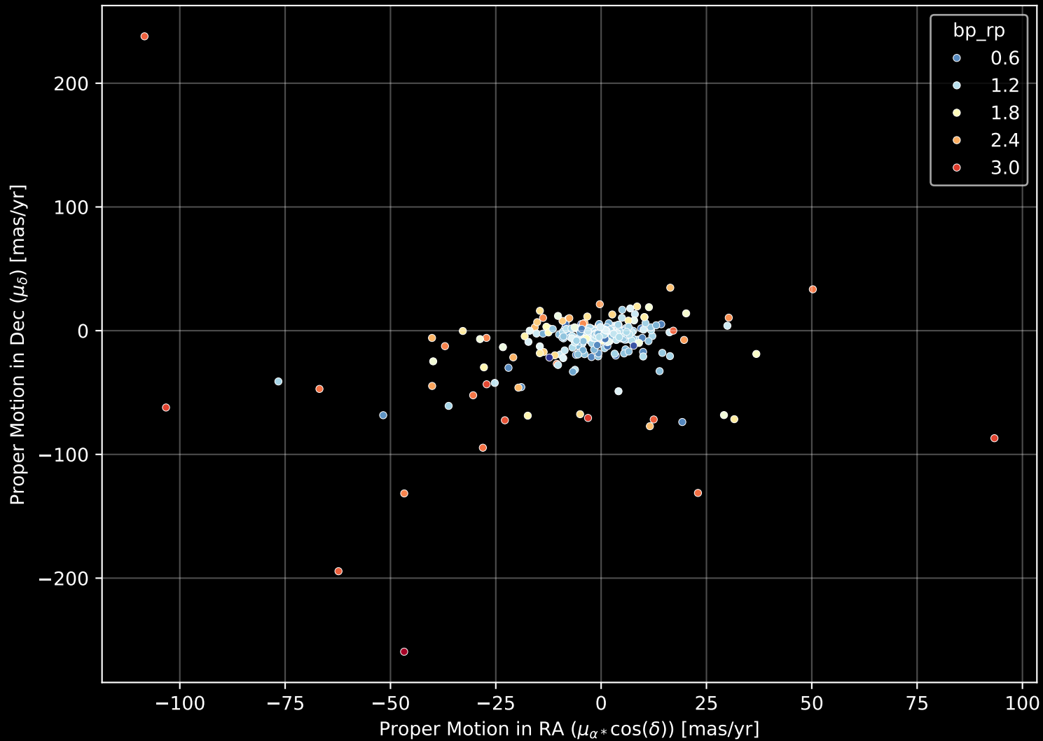
APOGEE DR17 Field: [150+30] Proper Motion Diagram (n= 404)
