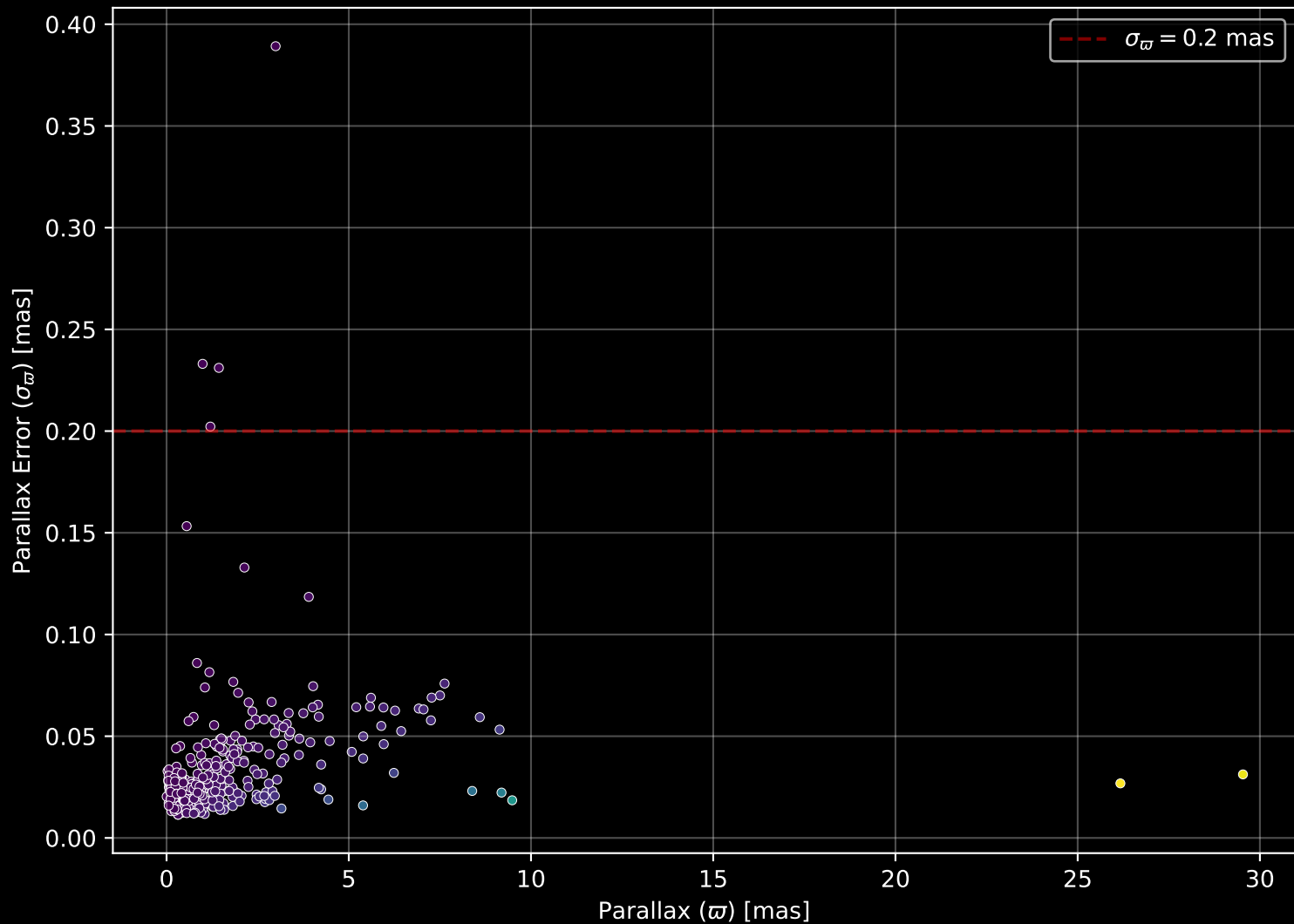
APOGEE DR17 Field: [150+30] Parallax Quality (n= 404)
